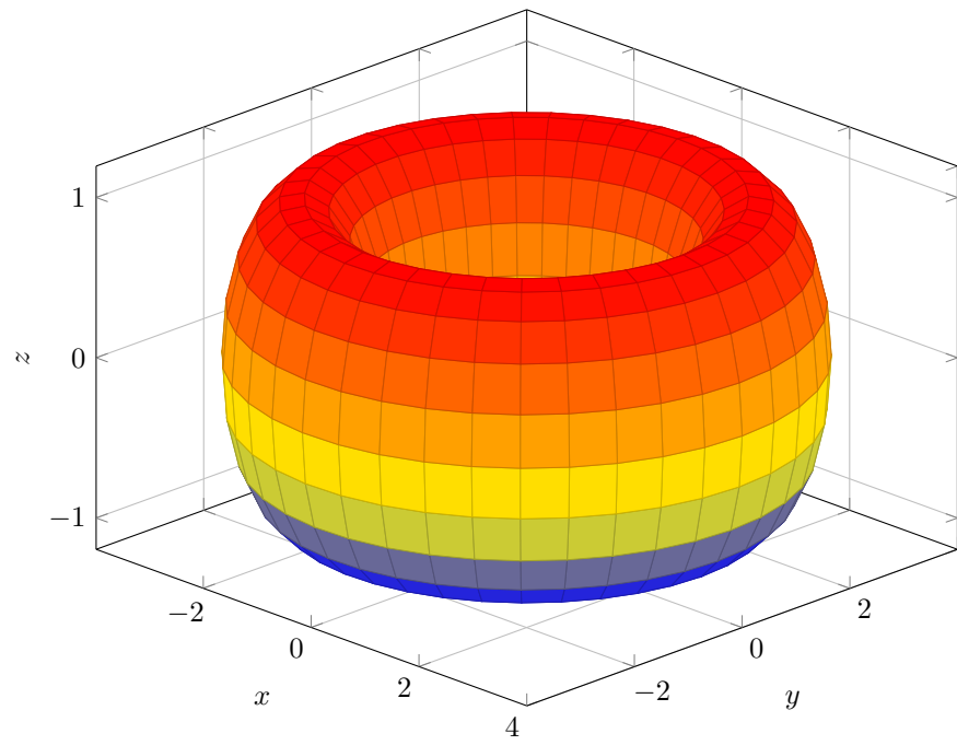
3D Parametric Plot of a Torus
