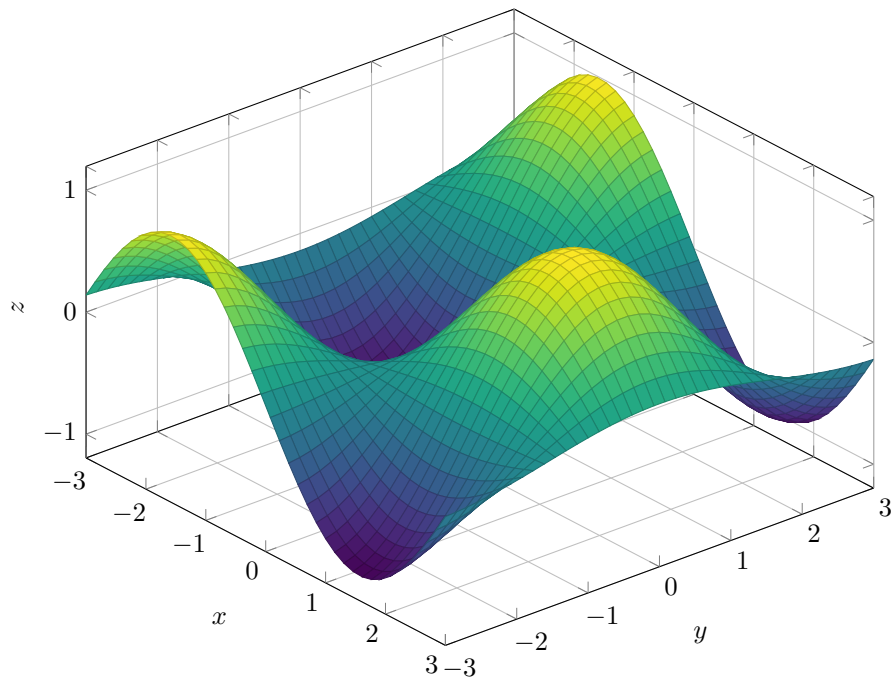
3D Surface Plot of \sin(x) \cdot \cos(y)
