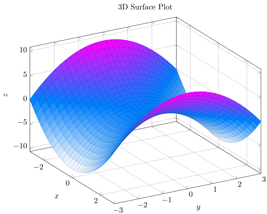
Figure 1: 3D Surface Plot of z = x^2 - y^2
